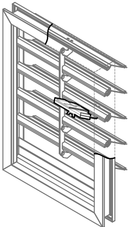
Heads and Jambs Cut Away for Clarity
