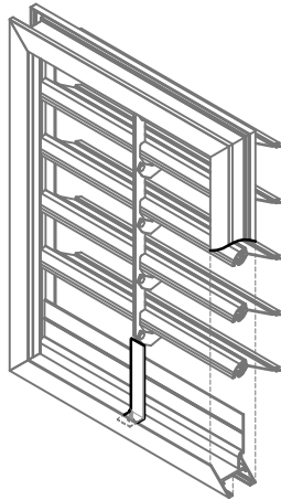
Jamb Cut Away for Clarity
