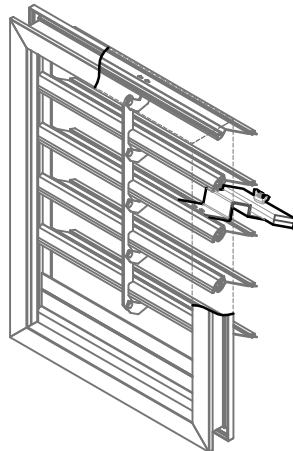
Heads and Jambs Cut Away for Clarity
